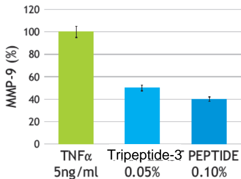
Inhibitory effect on MMP-9 release induced by TNF \alpha in HDF
